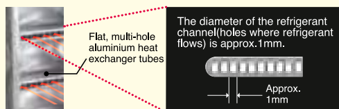
Flow of refrigerant
