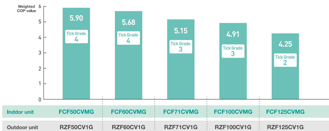
● Weighted COP value by capacity for cassette models
